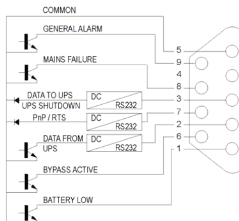
Рис.14:RS232/Interface
