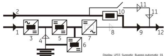
Display_LP33_Synoptic_Bypass automatic_01
